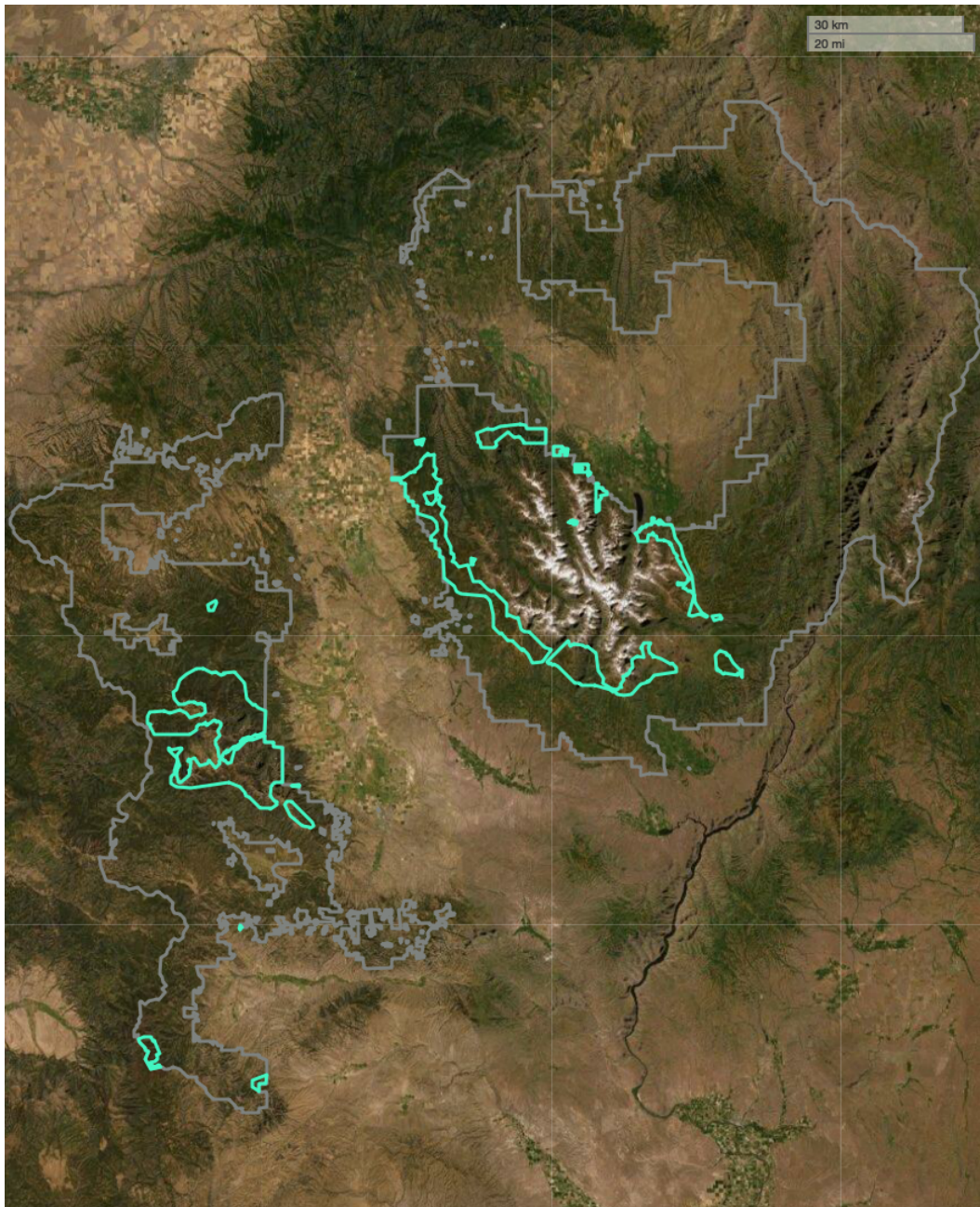
Figure C2. Satellite map of Wallowa-Whitman National Forest showing HEVAs (i.e., areas in the top 10% of ecological value) as green polygons. See the reference map (Fig. 2) for HEVA IDs, corresponding to rows in Table 1.
