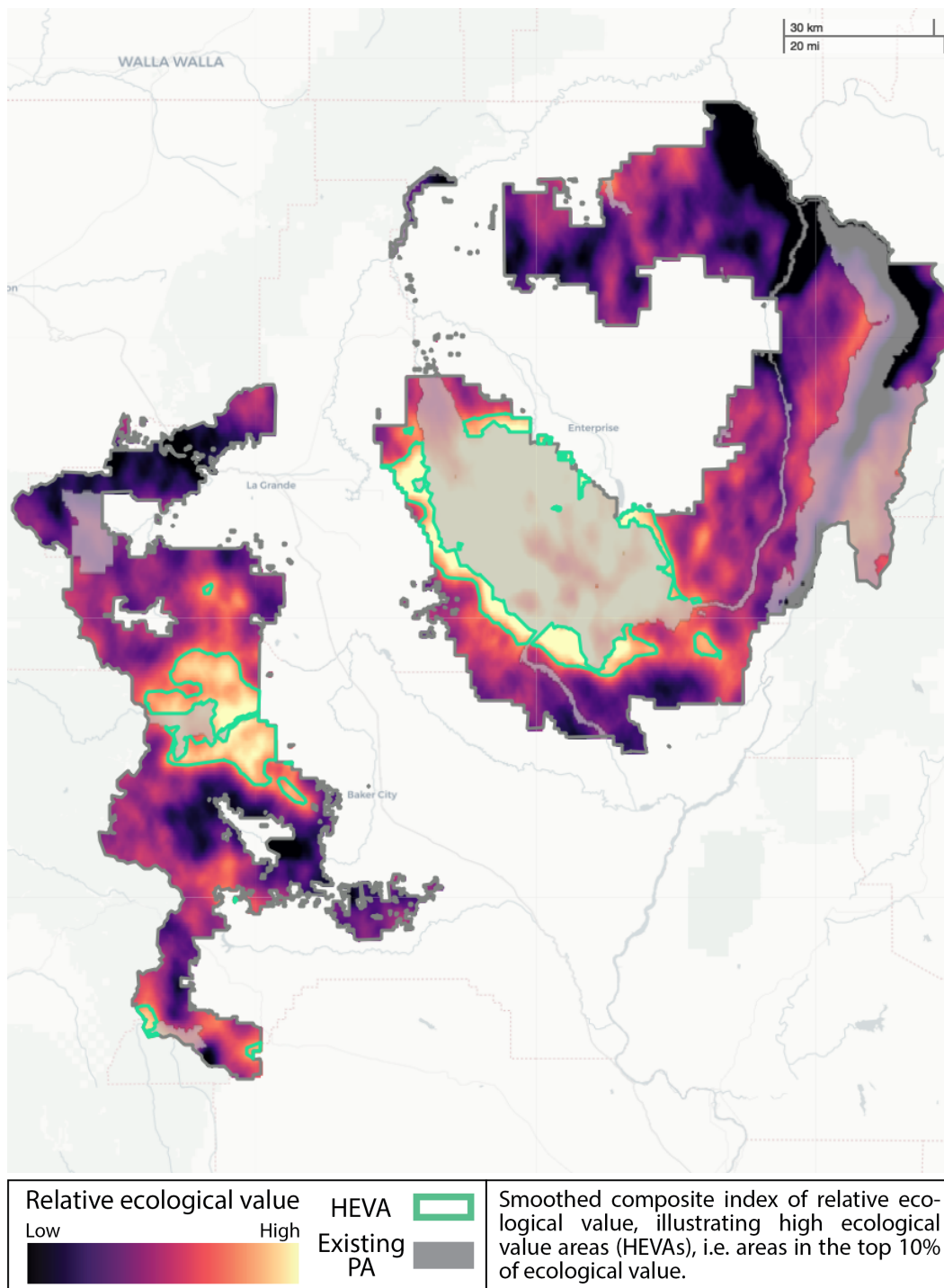
Figure 1. Map of Wallowa-Whitman National Forest showing the smoothed composite index of ecological value. See the reference map (Fig. 2) for HEVA labels, corresponding to rows in Table 1.
