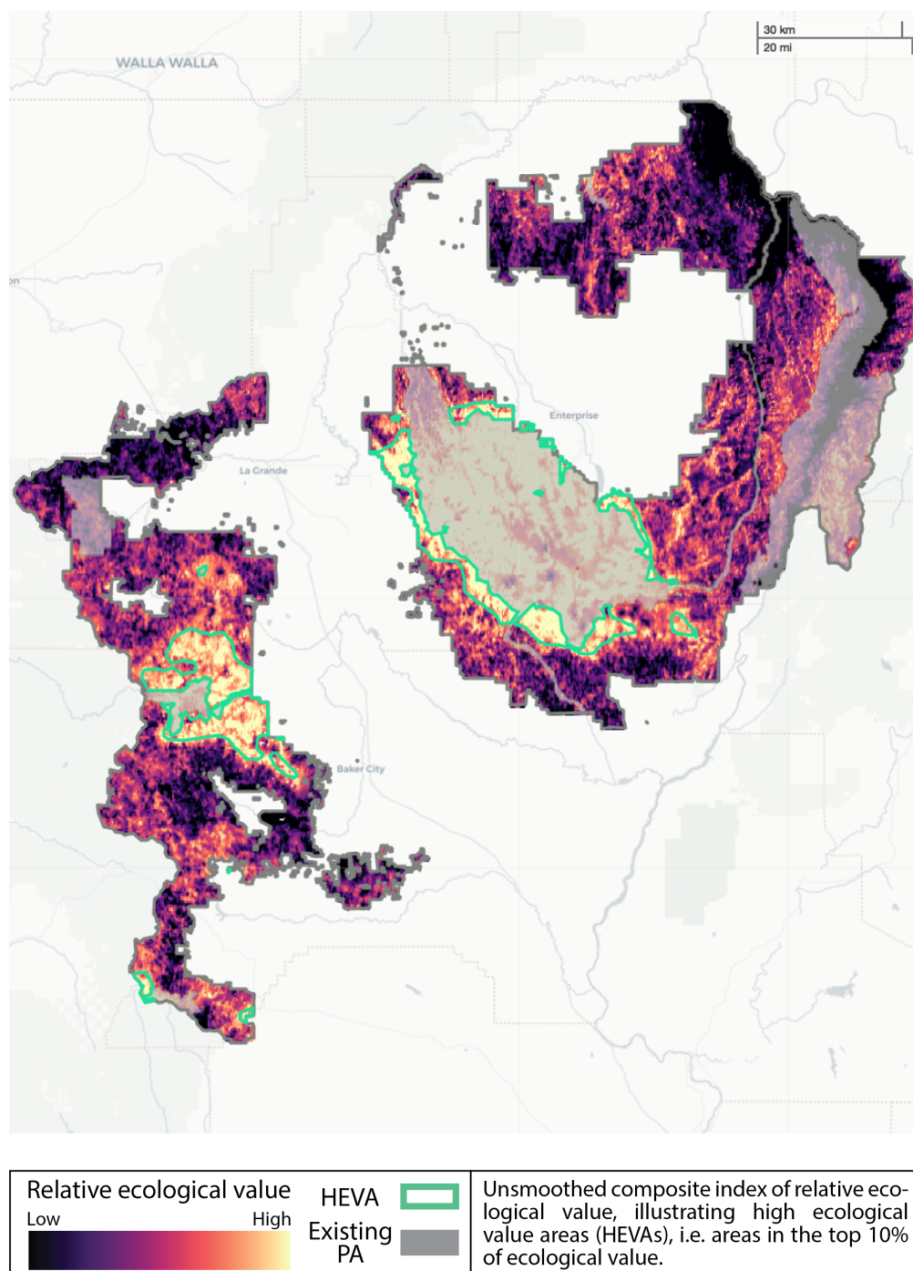
Figure C1. Map of Wallowa-Whitman National Forest showing the unsmoothed composite index of ecological value, with HEVAs (i.e., areas in the top 10% of ecological value) outlined in green. Existing protected areas (PAs) are shown as shaded gray regions. See the reference map (Fig. 2) for HEVA IDs, corresponding to rows in Table 1.
