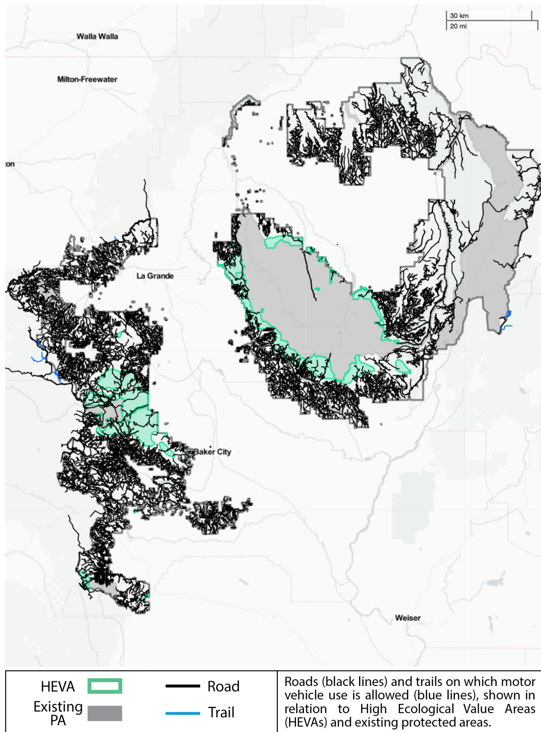
Figure C3. Map of Wallowa-Whitman National Forest showing roads and trails. See the reference map (Fig. 2) for HEVA IDs, corresponding to rows in Table 1.
