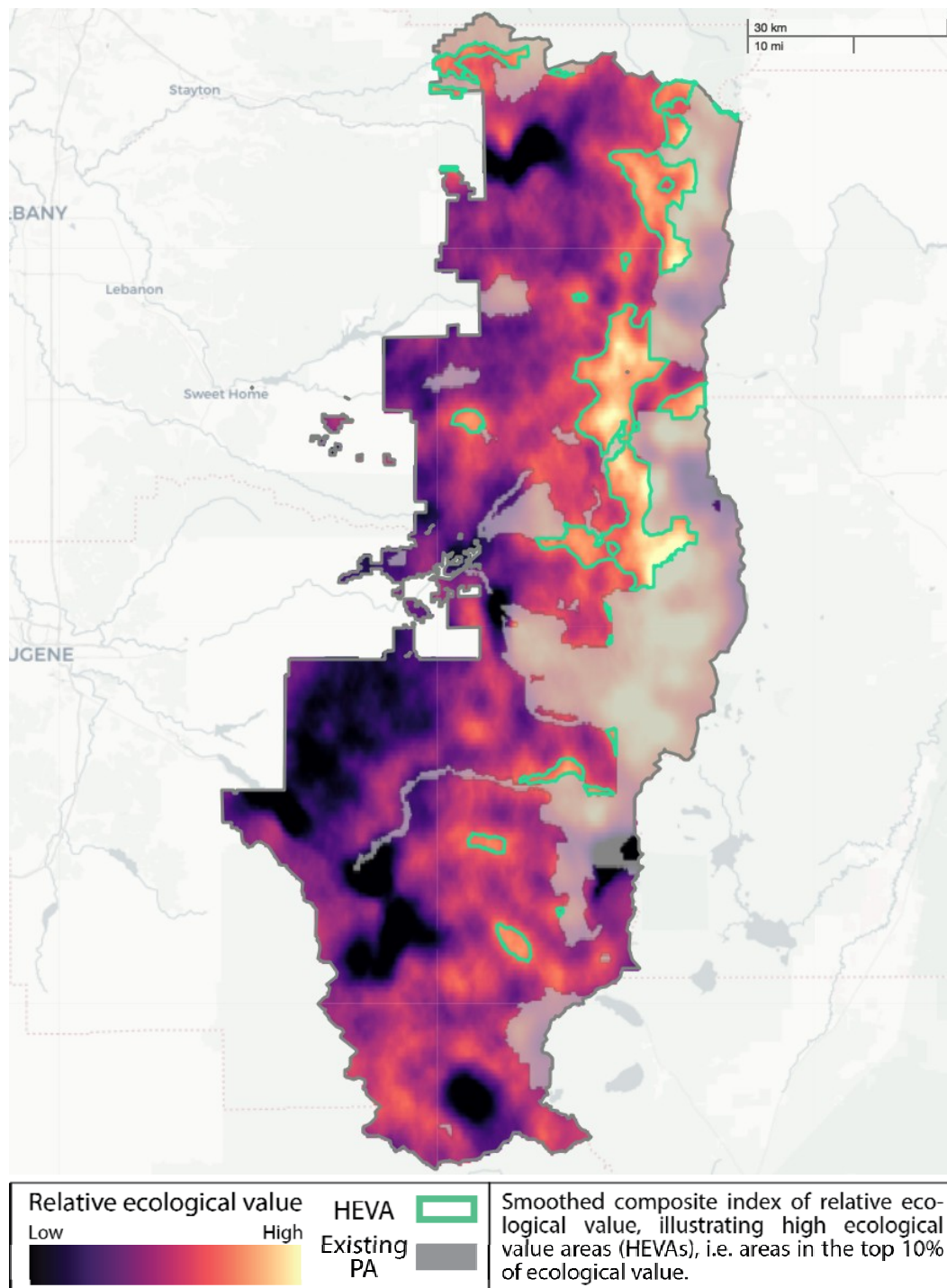
Figure 1. Map of Willamette National Forest showing the smoothed composite index of ecological value. See the reference map (Fig. 2) for HEVA labels, corresponding to rows in Table 1.
