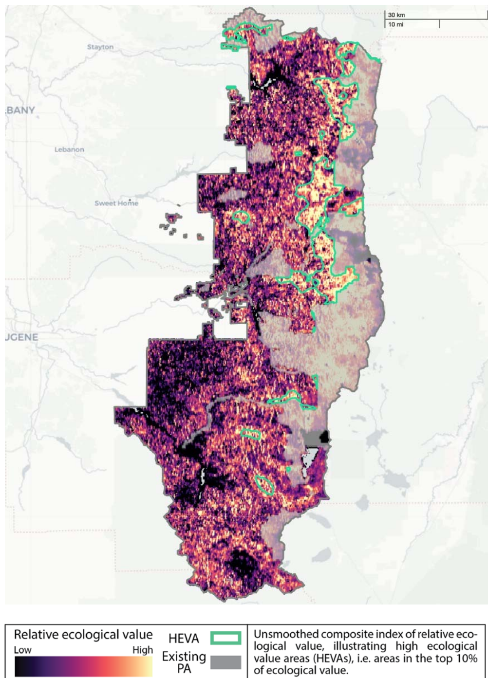
Figure C1. Map of Willamette National Forest showing the unsmoothed composite index of ecological value, with HEVAs (i.e., areas in the top 10% of ecological value) outlined in green. Existing protected areas (PAs) are shown as shaded gray regions. See the reference map (Fig. 2) for HEVA IDs, corresponding to rows in Table 1.
