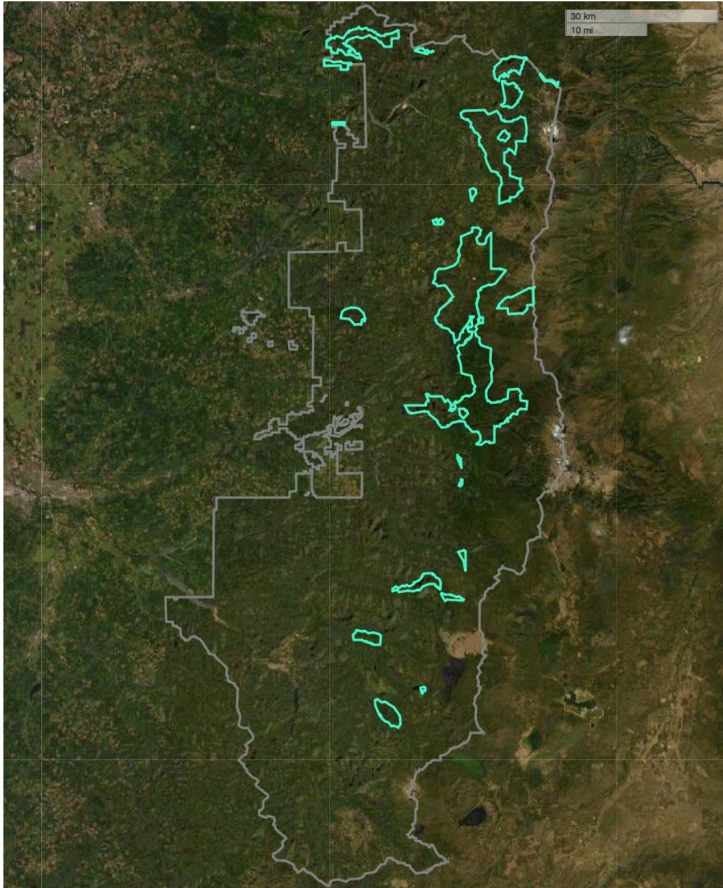
Figure C2. Satellite map of Willamette National Forest showing HEVAs (i.e., areas in the top 10% of ecological value) as green polygons. See the reference map (Fig. 2) for HEVA IDs, corresponding to rows in Table 1.
