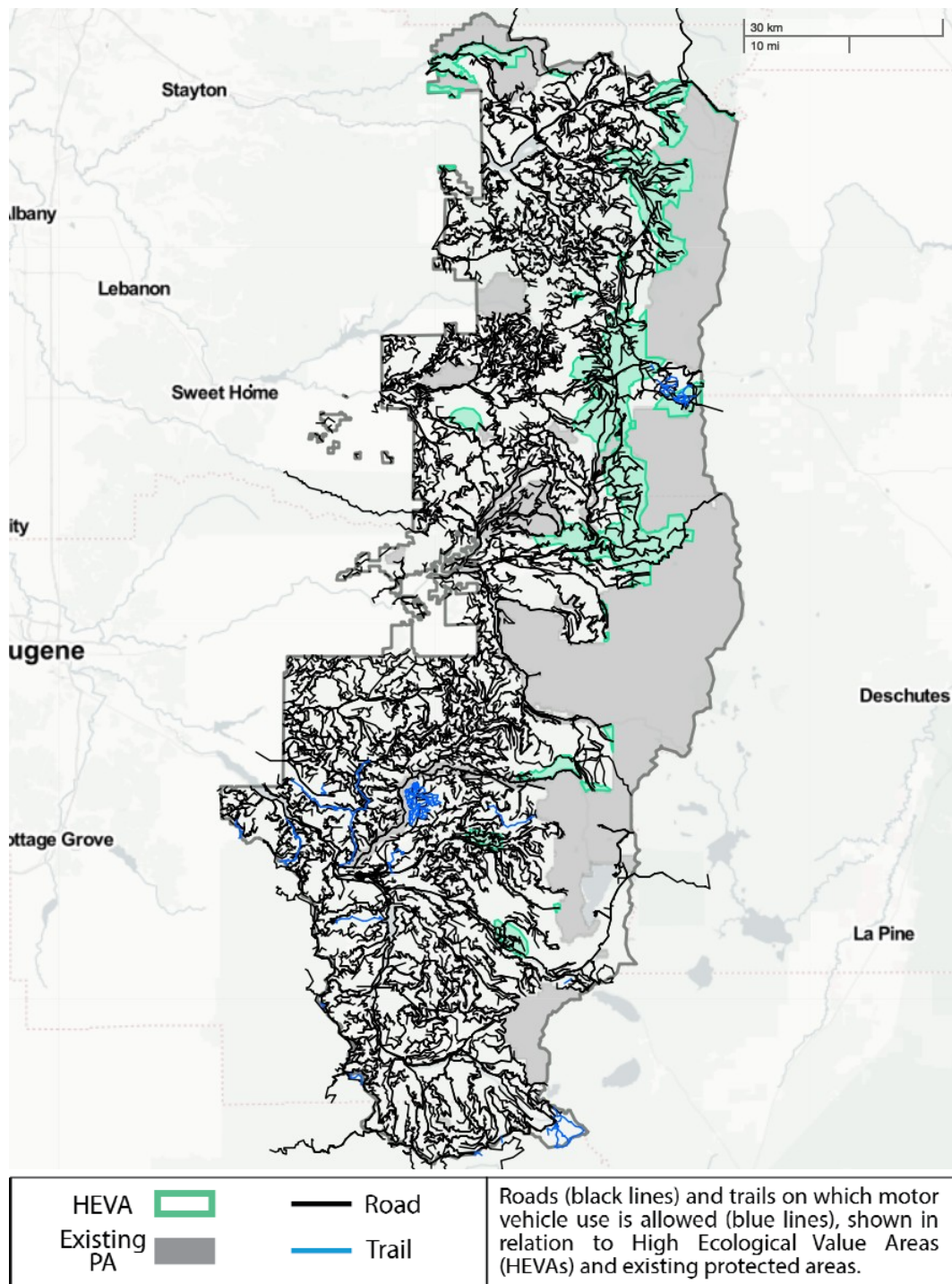
Figure C3. Map of Willamette National Forest showing roads and trails. See the reference map (Fig. 2) for HEVA IDs, corresponding to rows in Table 1.
